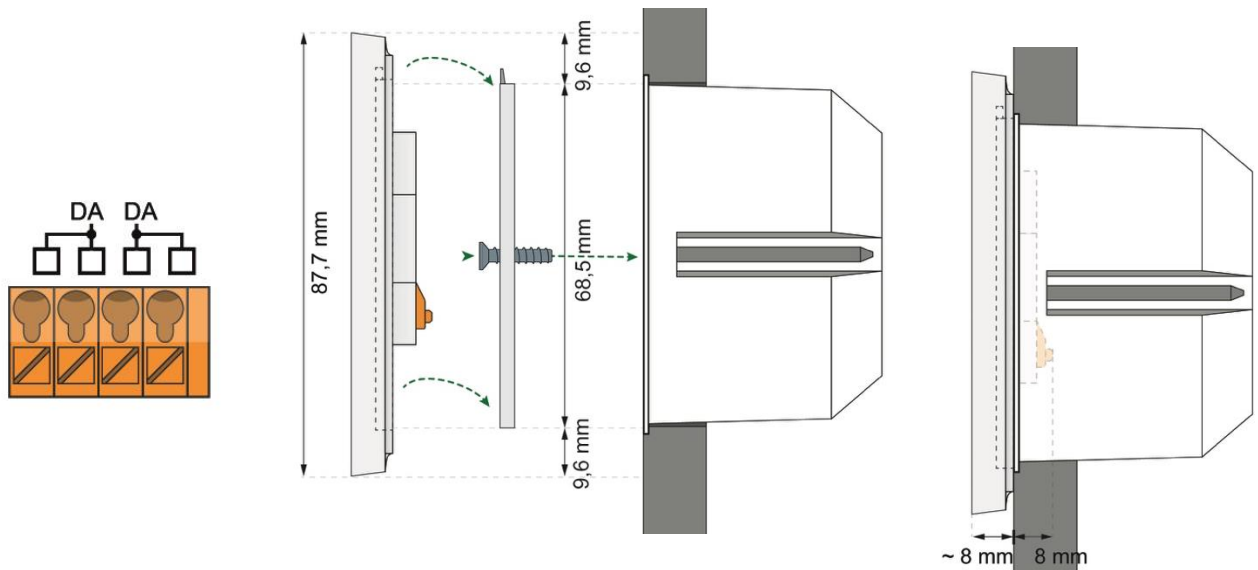
Abbildung 1 Installation: DALI-2 Touchpanel Touchpanel -> Montageplatte -> UP Dose
